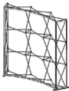
8-Foot Curved Frame 88 H x 91 W x D 21.25 (224 x 231 x 54 cm)
