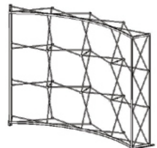
10-Foot Curved Frame 88 H x 118 W x 27.5 D (224 x 300 x 70 cm)
